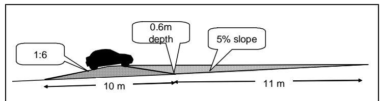
Figure 6—A cross-section of a whoa-boy on a 5 per cent slope assuming that there has been no cut and fill
