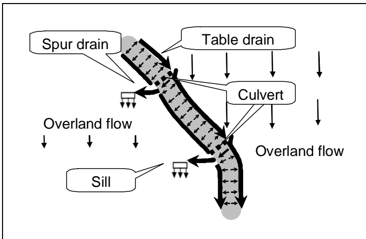
Figure 12—Spur drains collect runoff from table drains and culverts on a formed road
