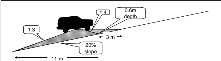
Figure 8—A 60 cm high whoa-boy constructed on a 20 per cent slope by importing road building material.
