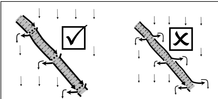
Figure 13—Correct and incorrect use of spur drains to remove runoff from a formed road
