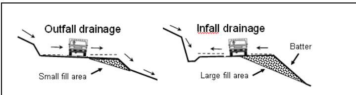
Figure 9—Outfall drainage removes runoff from the road and allows for the use of lower whoa-boys.
