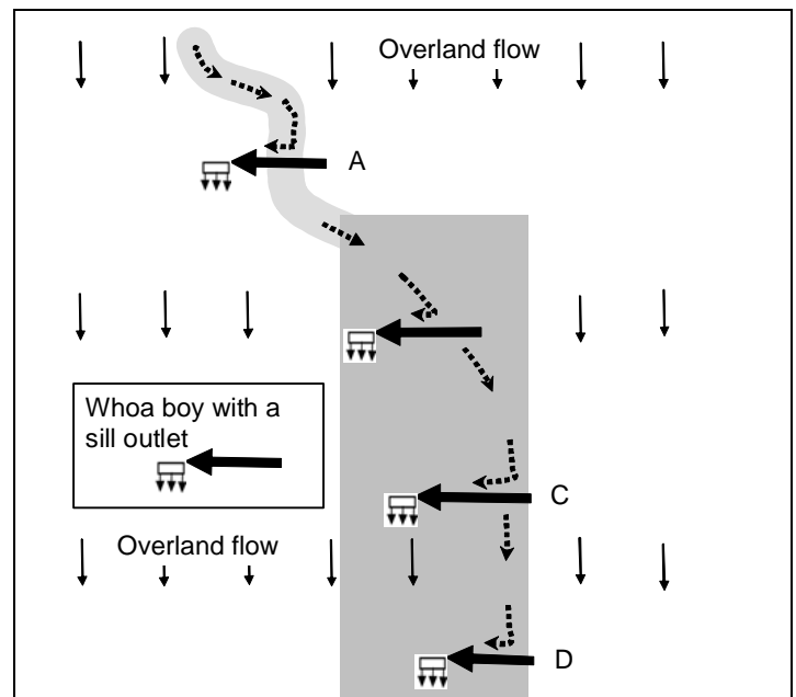
Figure 2—Using whoa-boys to allow overland flows to cross a road
