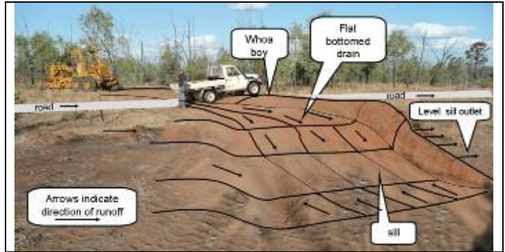
Figure 10—A whoa-boy with a sill outlet to spread runoff
